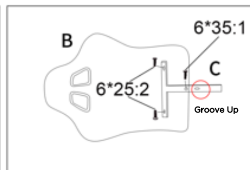
3. Install T-Bar to backrest chassis
