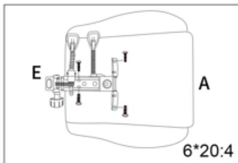
4. Install mechanism to under cushion
